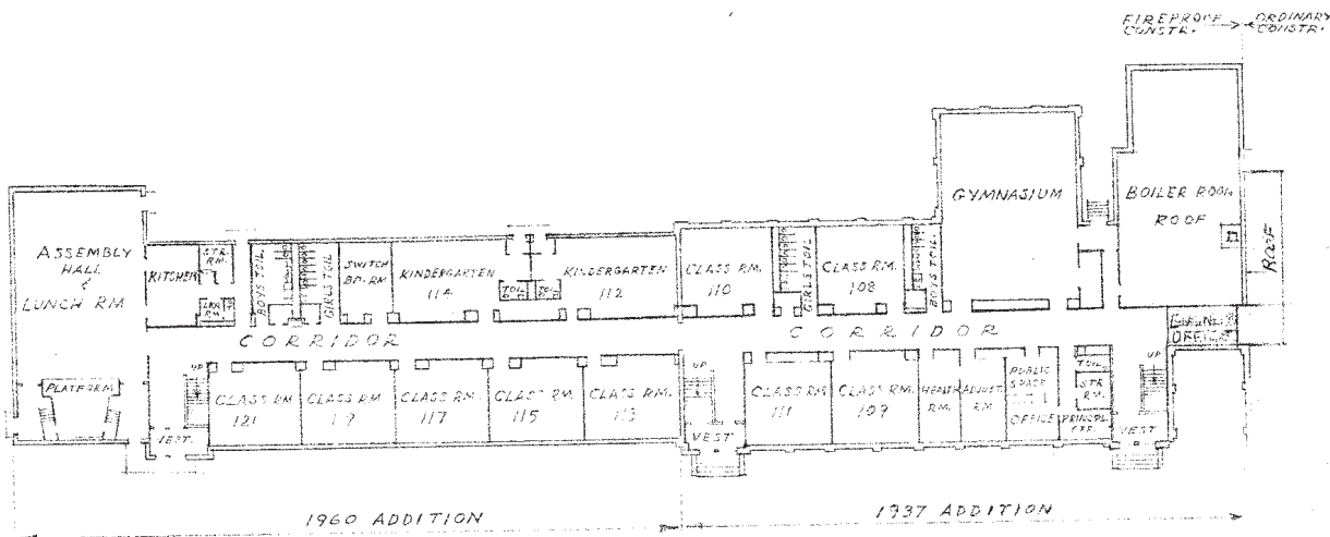
FIRST FLOOR PLAN SCALE 1"=50'-0"
